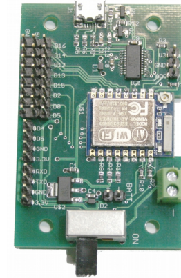
Switch in OFF position
